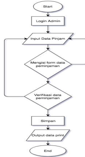
Gambar 3. Flowchart sistem
